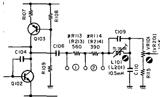
Fig. 6.12 16. Bias Trap (Playback)
