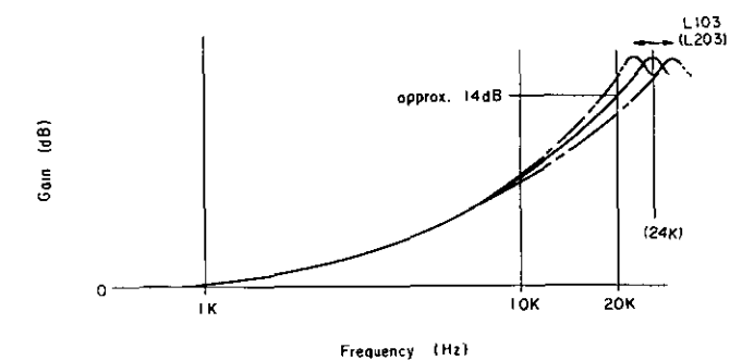
Fig. 6.16 Record Peaking Curve
